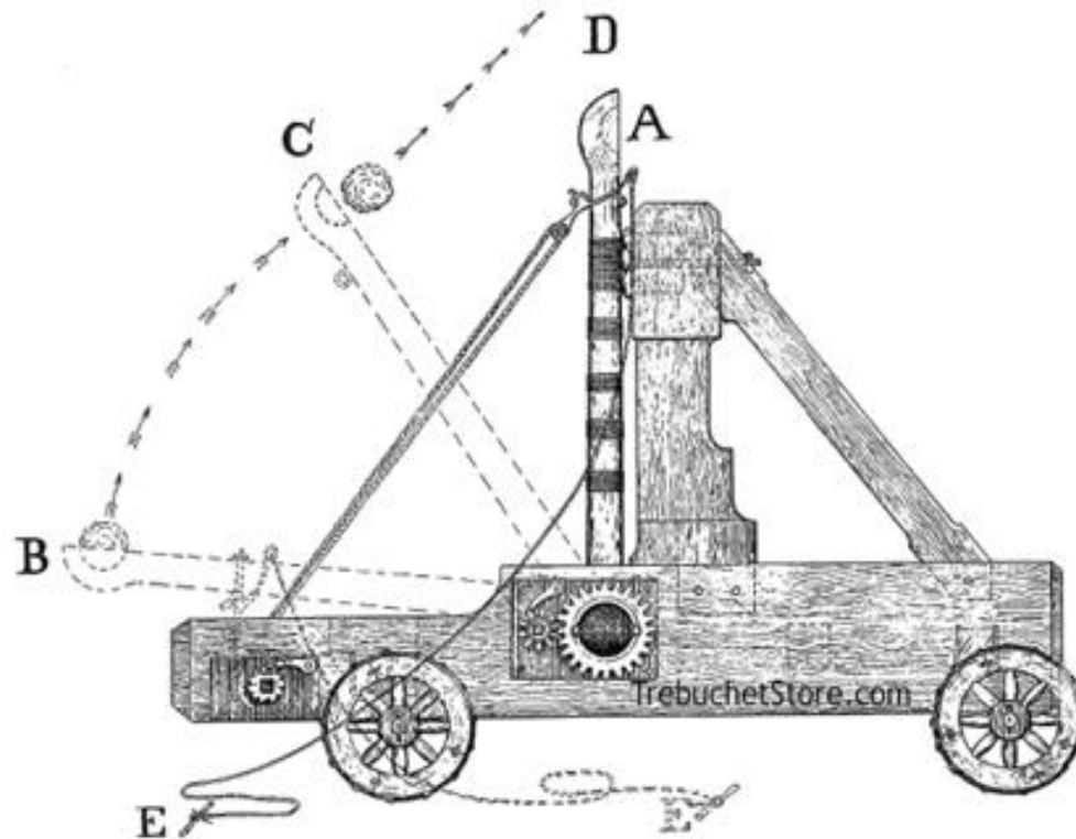
FIG. 194.—SIDE VIEW OF THE CATAPULT. Scale 1 in. = 1 ft.
